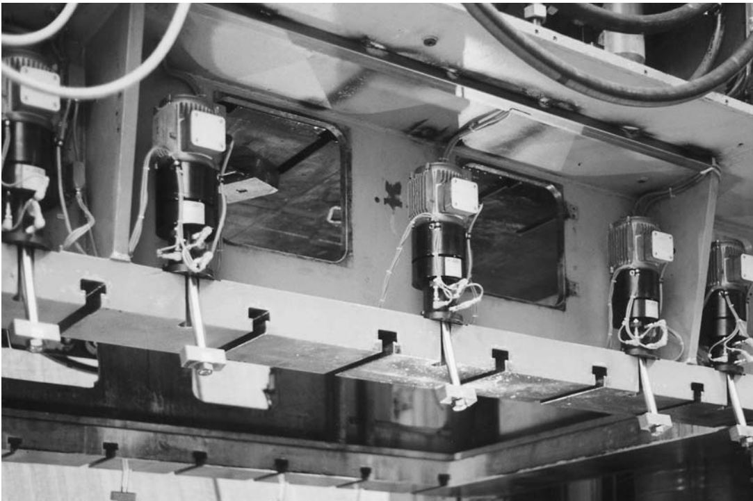
Electro-mechanical swing clamps mounted on a double-column press.
